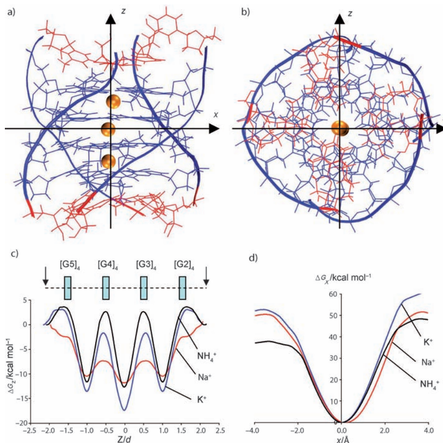
Figure 1. a) Side and b) top views of the K + form of the [d(TG 4 T)] 4 G-quadruplex structure. c) PMF profiles for ion movement inside the [d(TG 4 T)] 4 G-quadruplex channels. The arrows indicate the exit/entrance points of the channel. For easy comparison, a normalized reaction coordinate ( Z/d ) is used in the diagram where d is the averaged separation between two adjacent channel binding sites ( d = 2.71, 2.95 , and 3.09 Å for the Na + , K + , and NH 4 + forms of the G-quadruplex, respectively). d) Typical one-dimensional PMF profiles for the "sideways" ion movement inside the channel ( Z = 0 and along the x axis). See the Supporting Information for a complete set of 2D PMF profiles.
