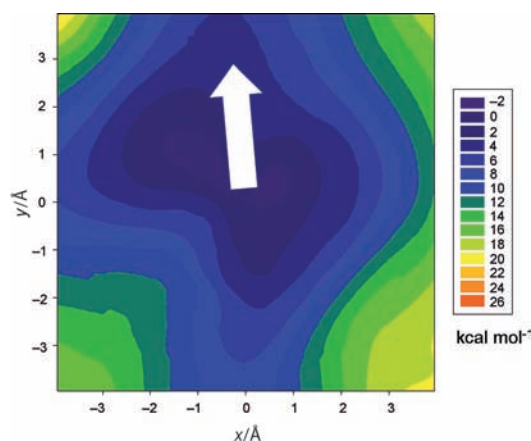
Figure 2. A typical 2D PMF landscape for K + movement in the XY plane at the exit/entrance points. The arrow indicates the least resistant pathway for ion movement away from the channel axis ( X = 0 and Y = 0 ) toward bulk solution. In this case, the Z position was chosen to be approximately 2.3 Å above the 5'-end G-quartet, [G2] 4 as defined in Figure 1c.
